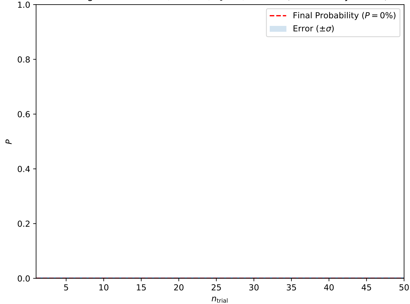
Convergence at A = 0.7, H = 0.5, T_0 = 1, w = 7.5 (Isolated Skyrmions)
