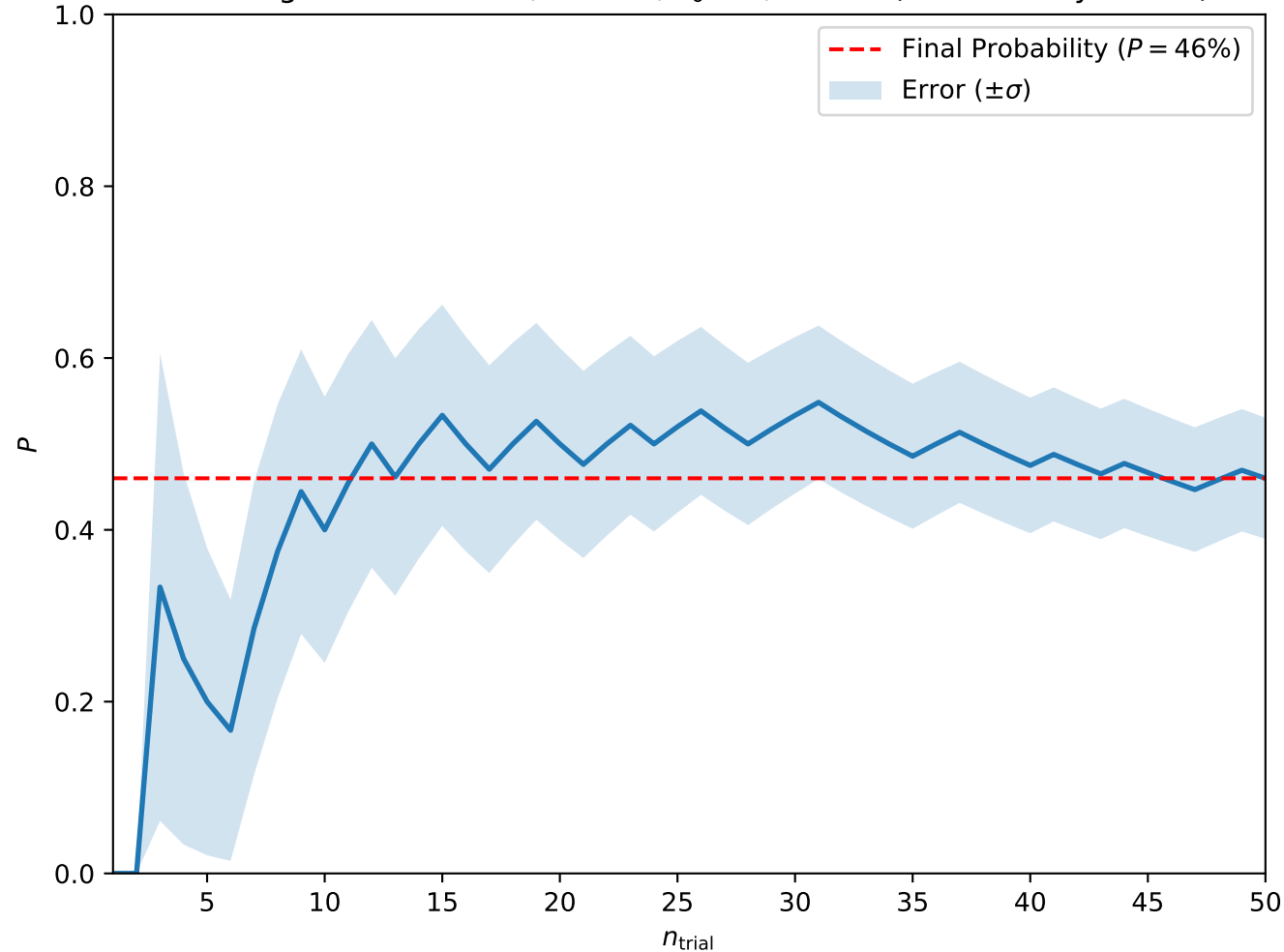
Convergence at A = 0.7, H = 0.5, T_0 = 3, w = 10 (Isolated Skyrmions)
