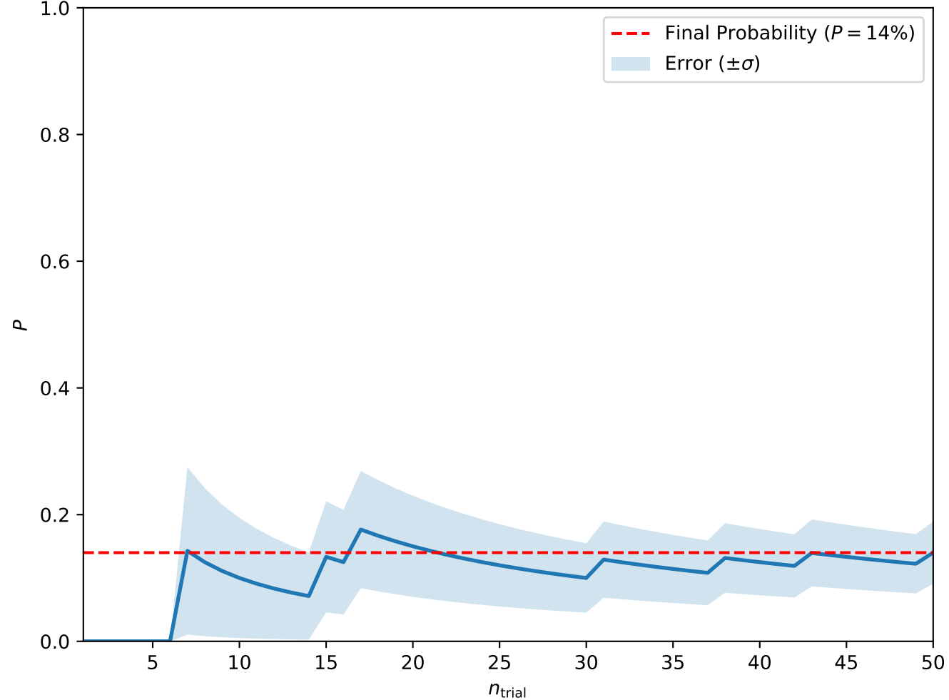
Convergence at A = 0.7, H = 0.5, T_0 = 3, w = 5 (Isolated Skyrmions)
