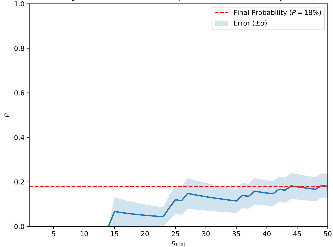
Convergence at A = 0.7, H = 0.5, T_0 = 3, w = 7.5 (Isolated Skyrmions)
