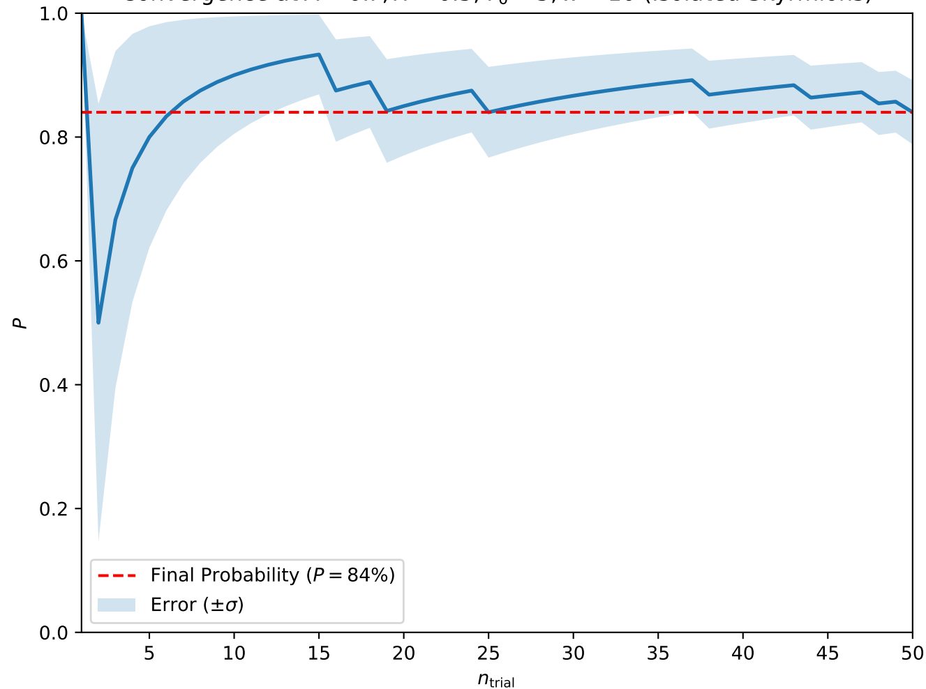
Convergence at A = 0.7, H = 0.5, T_0 = 5, w = 10 (Isolated Skyrmions)
