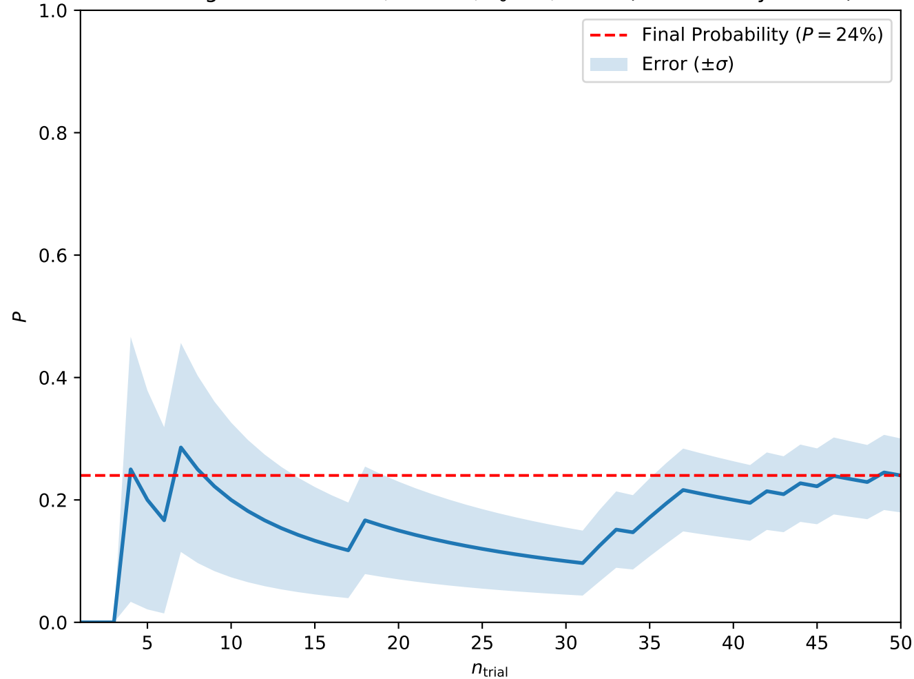
Convergence at A = 0.7, H = 0.5, T_0 = 5, w = 5 (Isolated Skyrmions)
