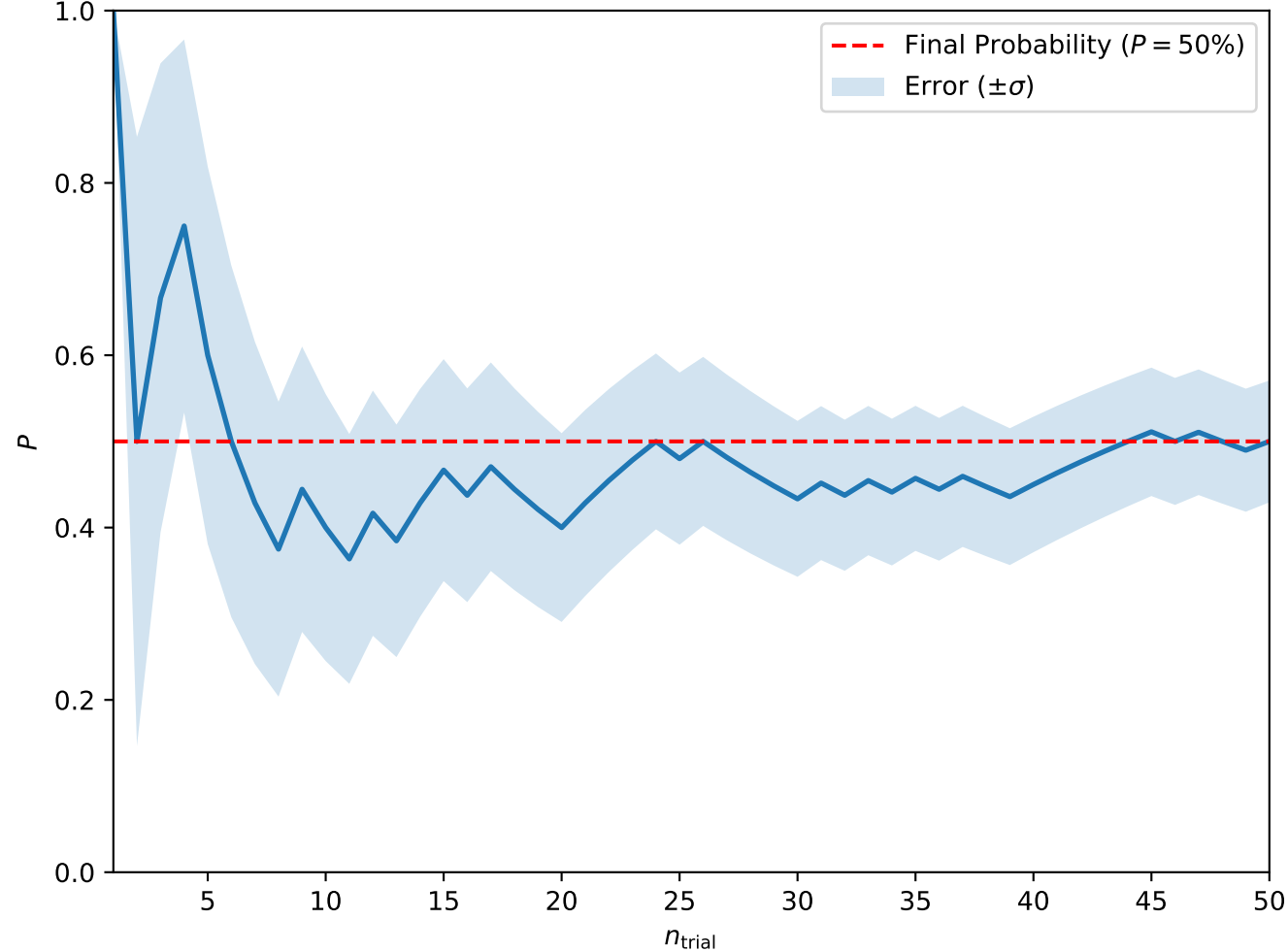
Convergence at A = 0.7, H = 0.5, T_0 = 5, w = 7.5 (Isolated Skyrmions)
