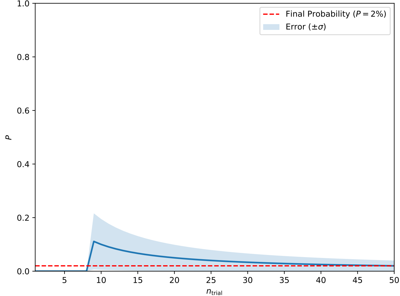
Convergence at A = 0.8, H = 0.3, T_0 = 1, w = 2.5 (Isolated Skyrmions)
