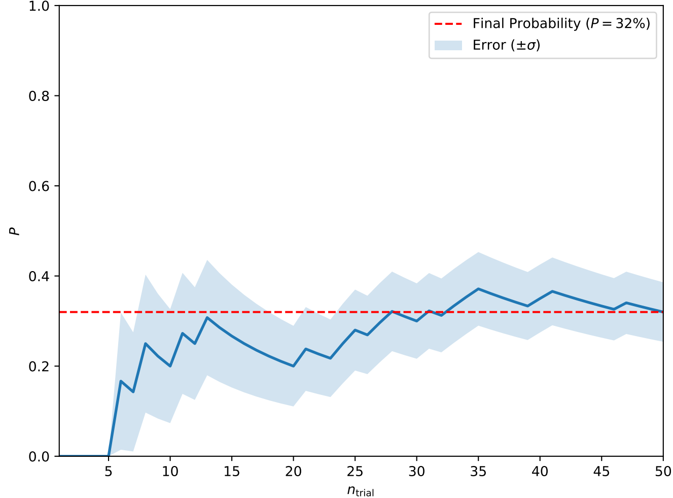
Convergence at A = 0.8, H = 0.3, T_0 = 1, w = 5 (Isolated Skyrmions)
