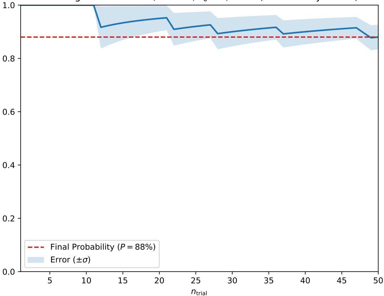
Convergence at A = 0.8, H = 0.3, T_0 = 3, w = 5 (Isolated Skyrmions)
