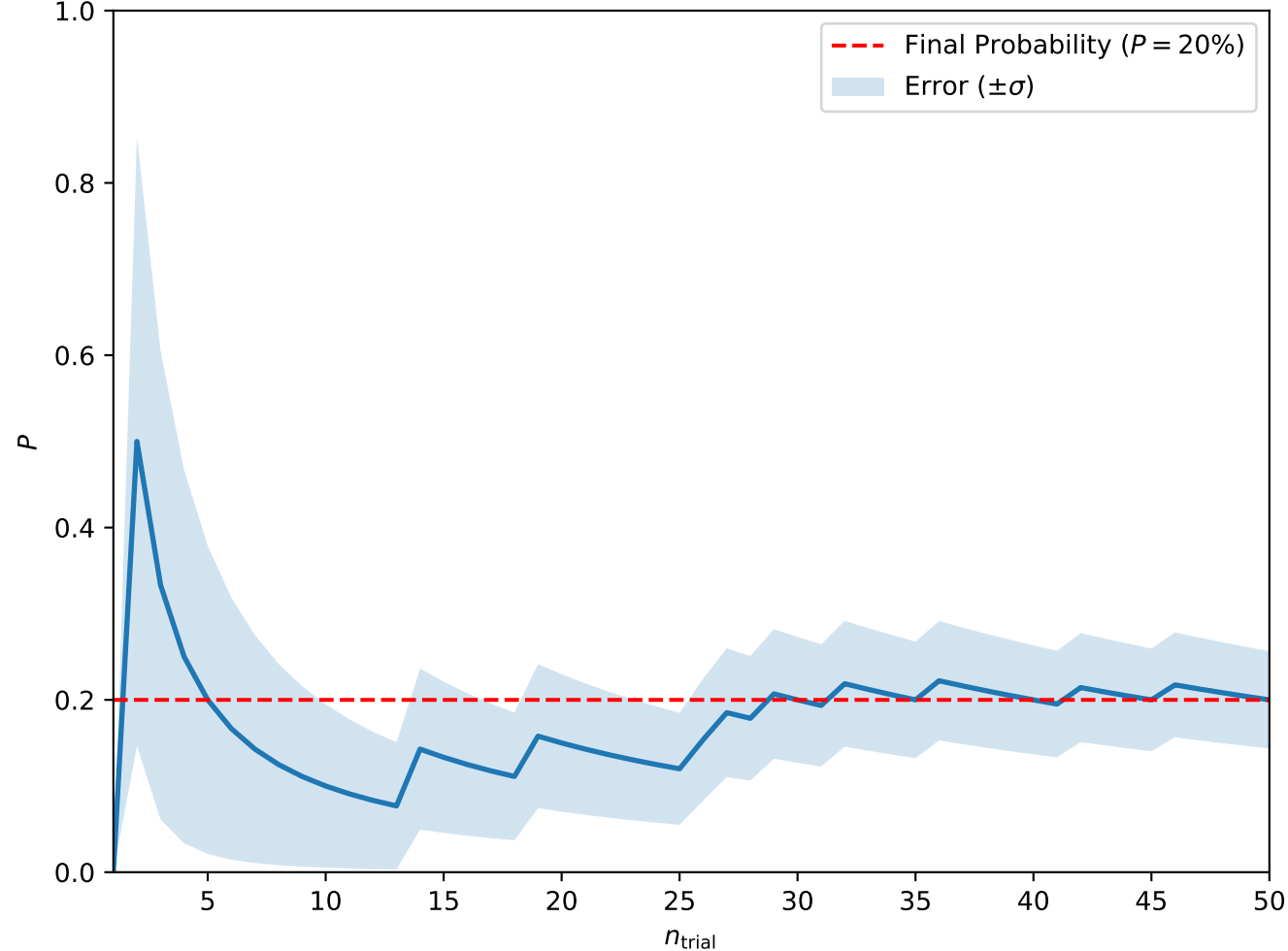
Convergence at A = 0.8, H = 0.3, T_0 = 5, w = 2.5 (Isolated Skyrmions)
