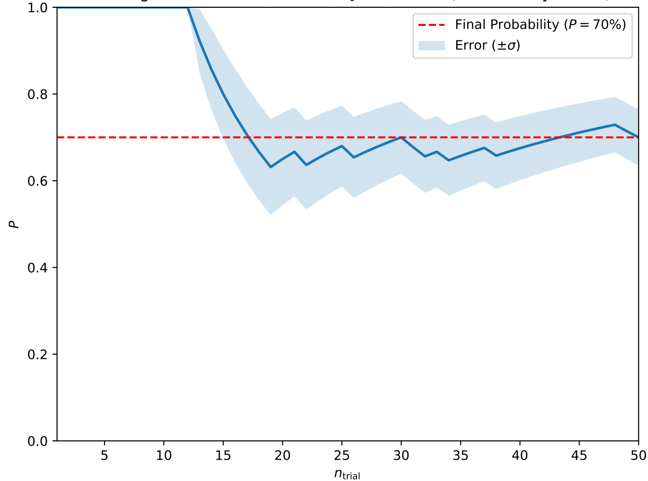
Convergence at A = 0.8, H = 0.4, T_0 = 1, w = 10 (Isolated Skyrmions)
