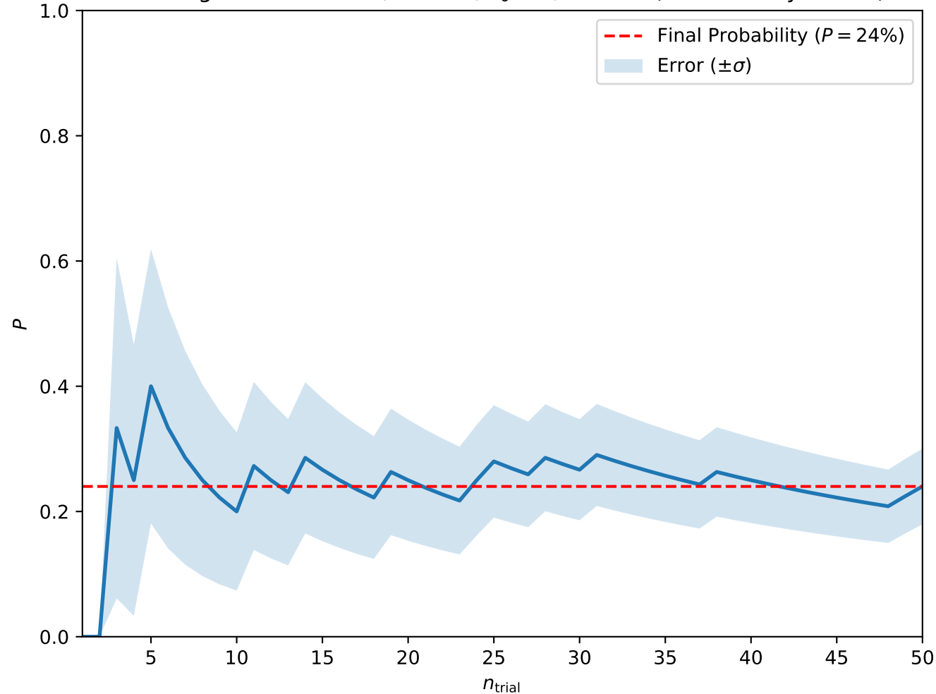
Convergence at A = 0.8, H = 0.4, T_0 = 1, w = 7.5 (Isolated Skyrmions)
