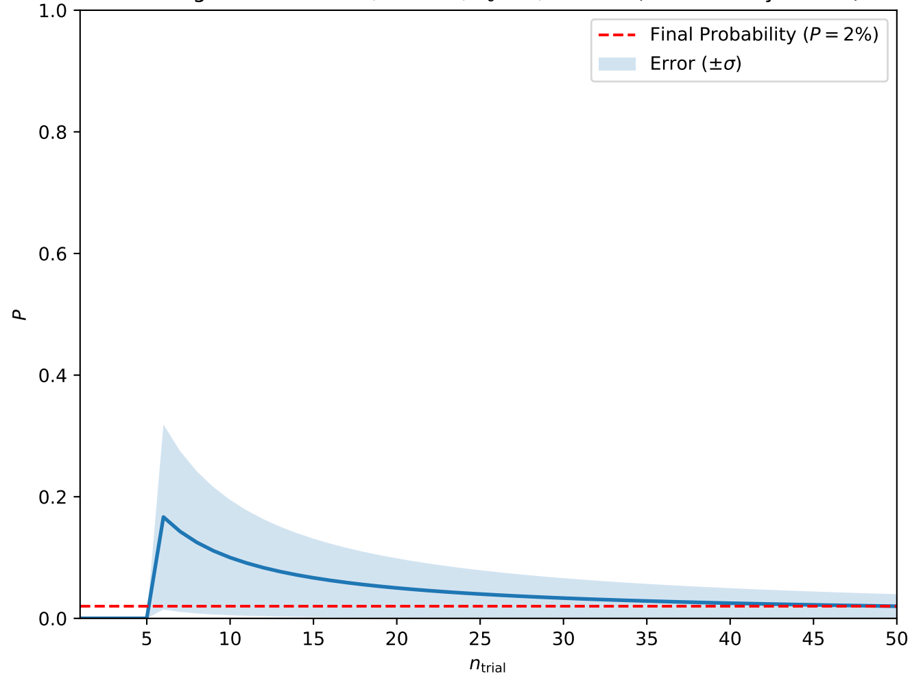
Convergence at A = 0.8, H = 0.4, T_0 = 3, w = 2.5 (Isolated Skyrmions)
