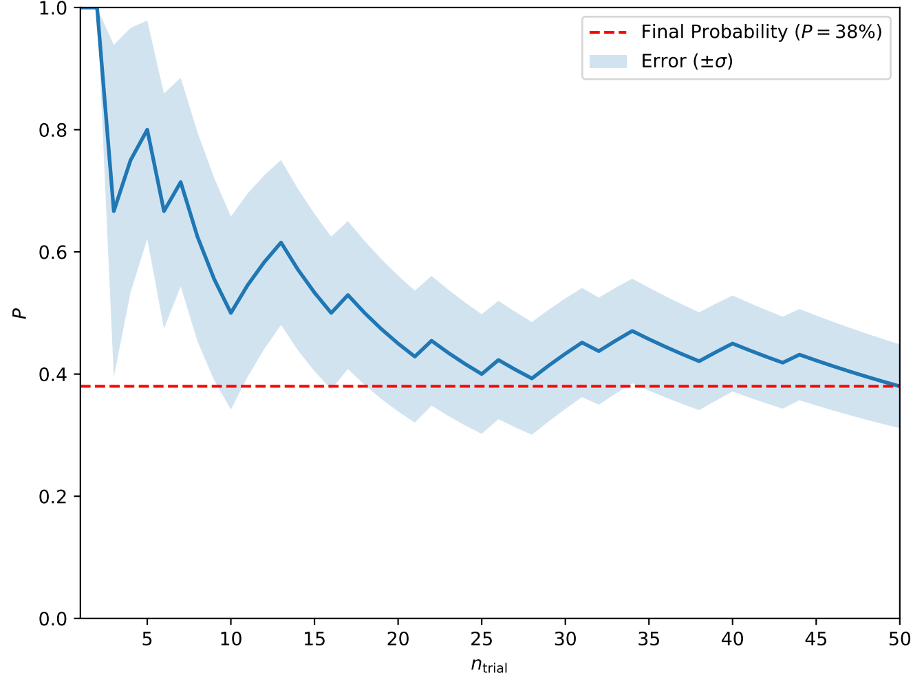
Convergence at A = 0.8, H = 0.4, T_0 = 3, w = 5 (Isolated Skyrmions)
