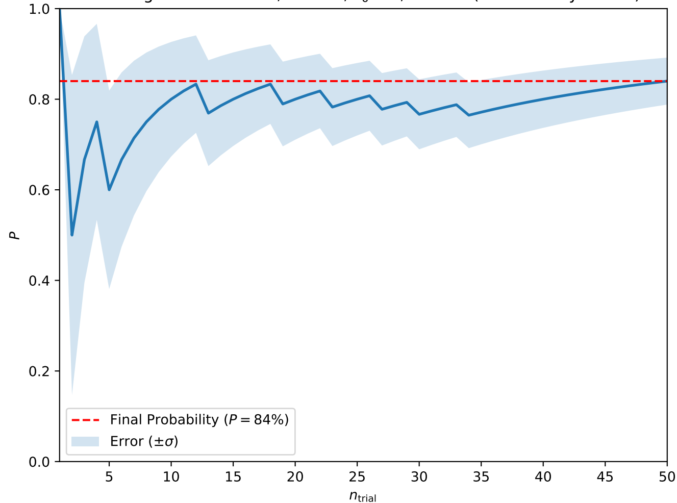
Convergence at A = 0.8, H = 0.4, T_0 = 3, w = 7.5 (Isolated Skyrmions)
