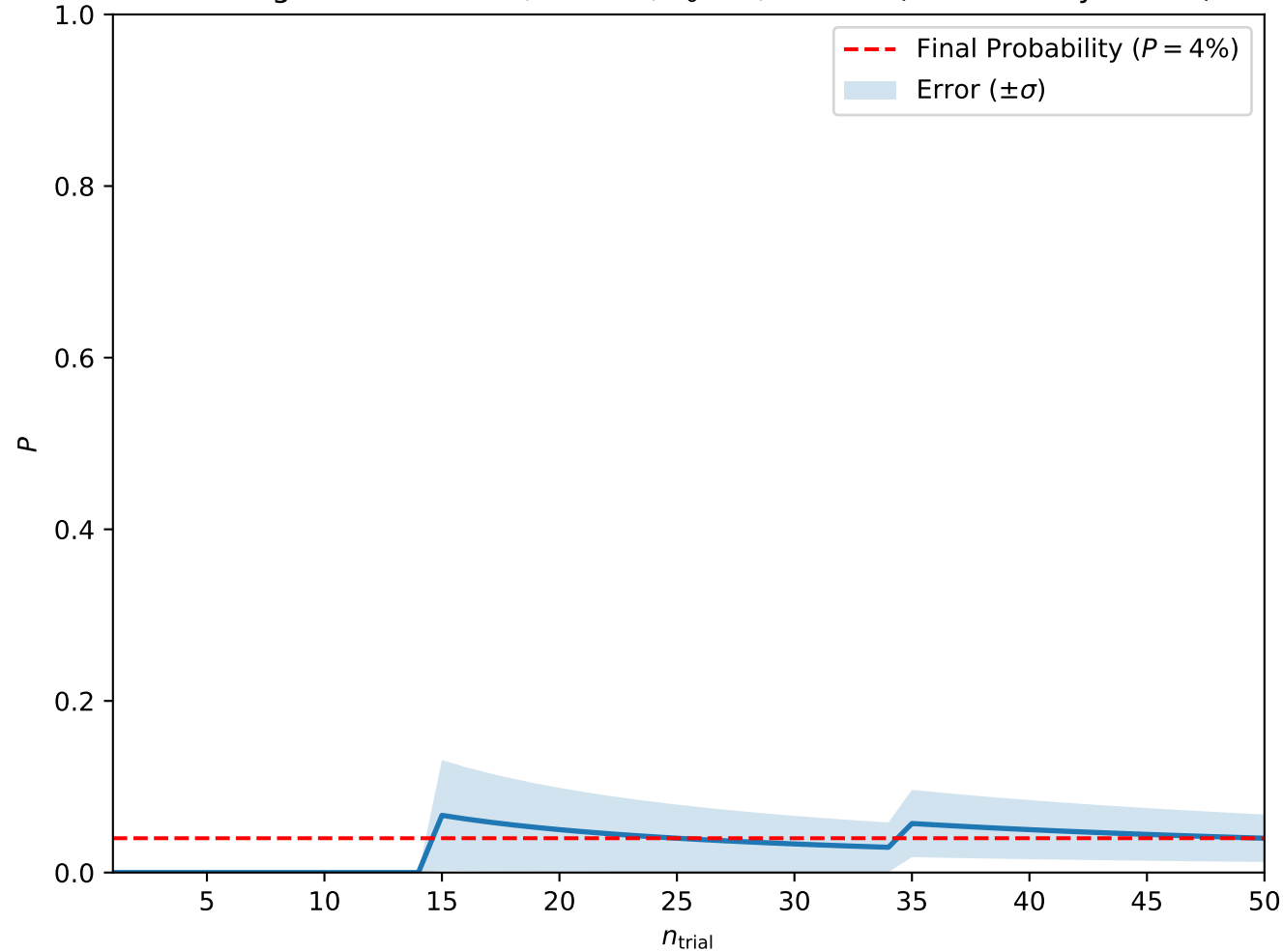
Convergence at A = 0.8, H = 0.4, T_0 = 5, w = 2.5 (Isolated Skyrmions)
