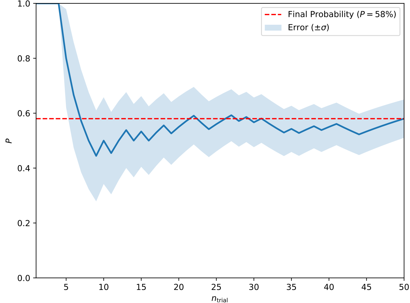
Convergence at A = 0.8, H = 0.4, T_0 = 5, w = 5 (Isolated Skyrmions)
