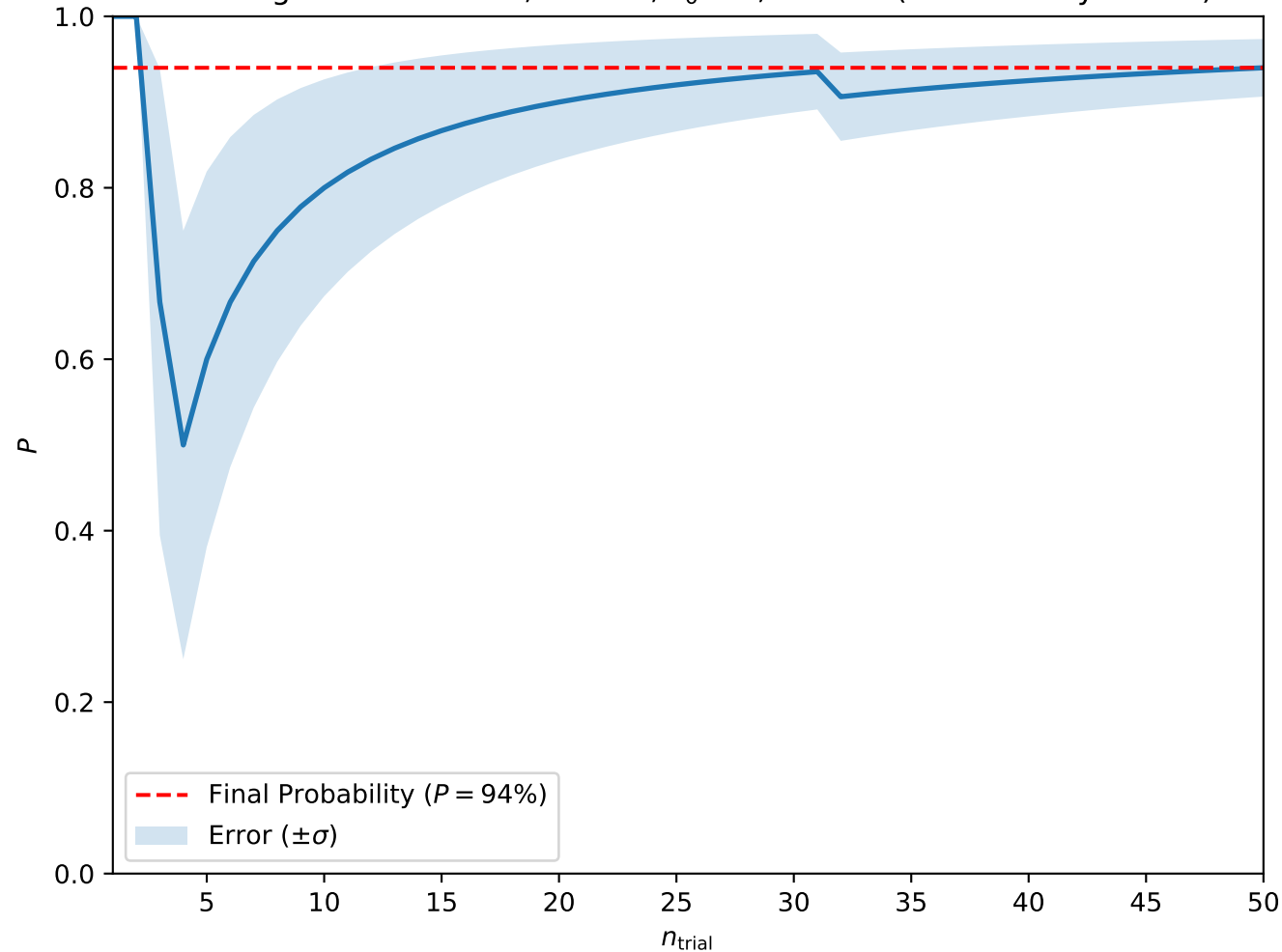
Convergence at A = 0.8, H = 0.4, T_0 = 5, w = 7.5 (Isolated Skyrmions)
