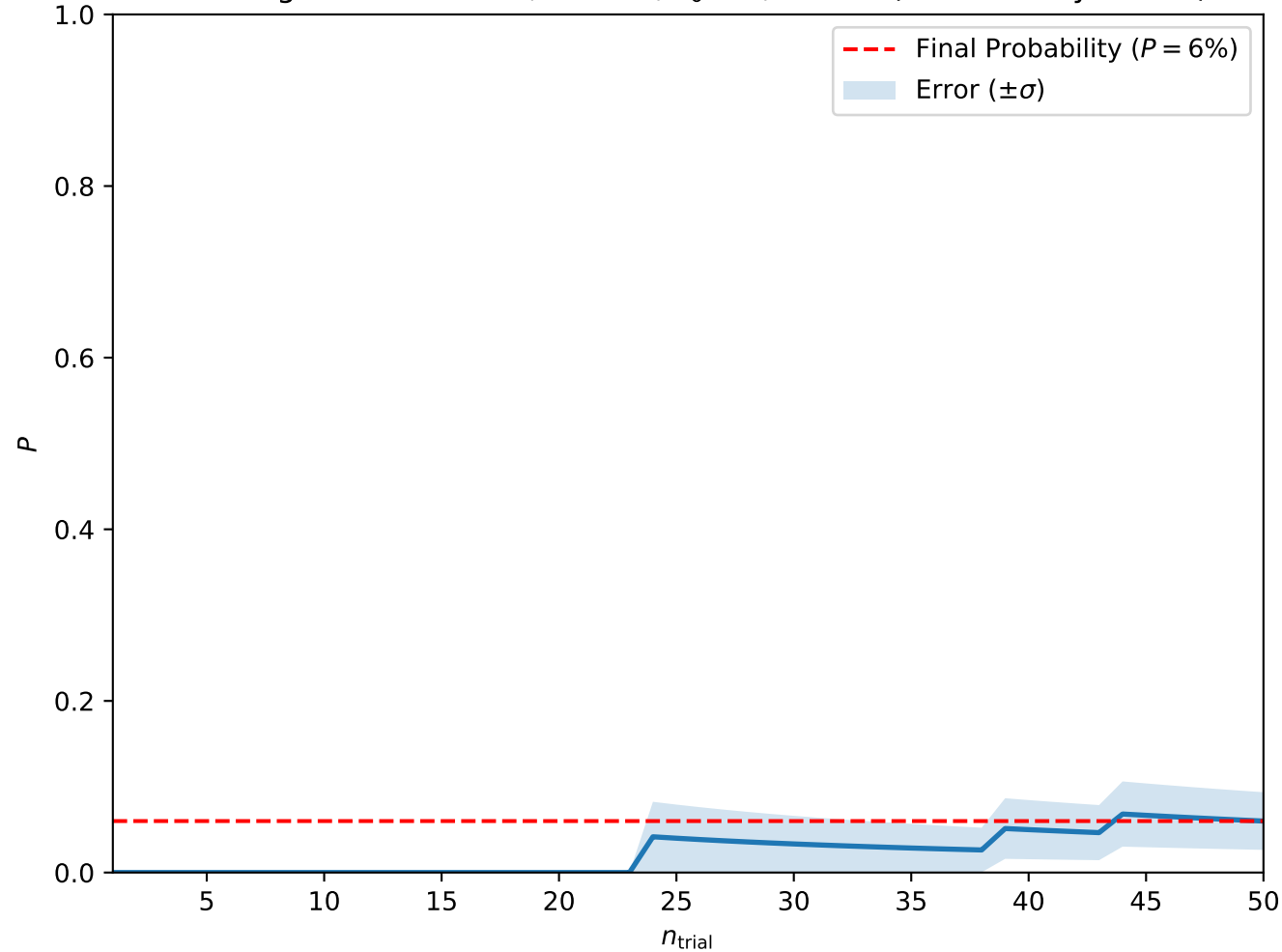
Convergence at A = 0.8, H = 0.5, T_0 = 1, w = 10 (Isolated Skyrmions)
