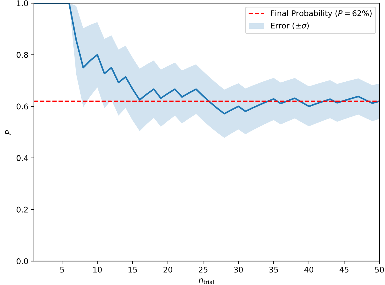
Convergence at A = 0.8, H = 0.5, T_0 = 3, w = 10 (Isolated Skyrmions)
