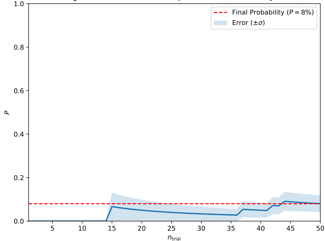
Convergence at A = 0.8, H = 0.5, T_0 = 3, w = 5 (Isolated Skyrmions)
