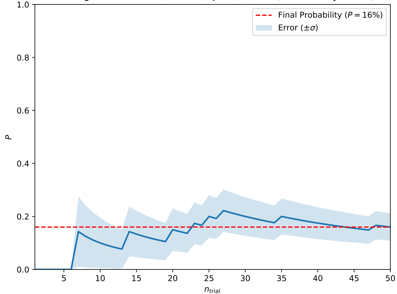
Convergence at A = 0.8, H = 0.5, T_0 = 3, w = 7.5 (Isolated Skyrmions)
