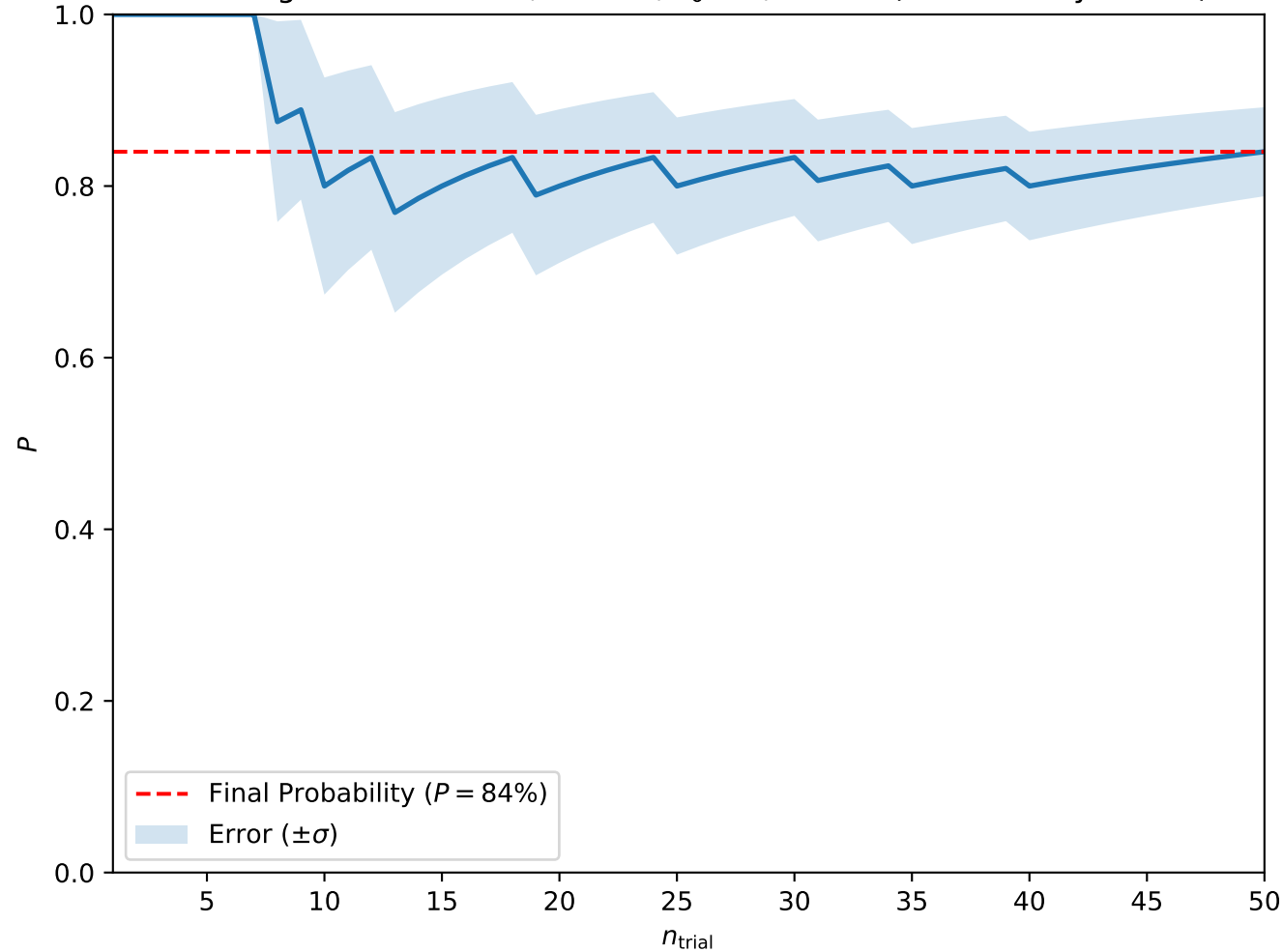
Convergence at A = 0.8, H = 0.5, T_0 = 5, w = 10 (Isolated Skyrmions)
