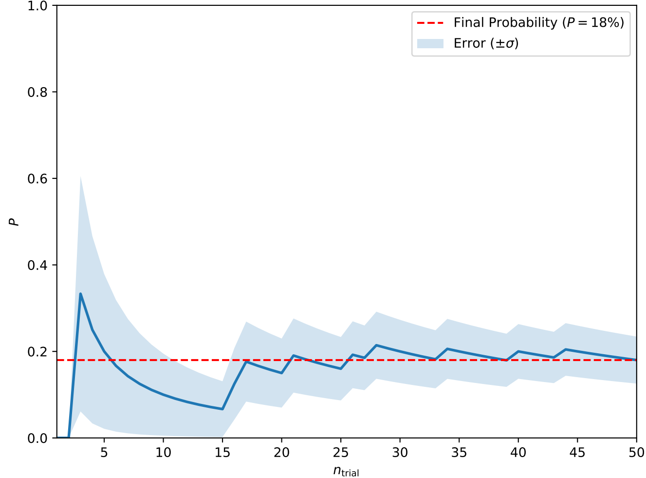
Convergence at A = 0.8, H = 0.5, T_0 = 5, w = 5 (Isolated Skyrmions)
