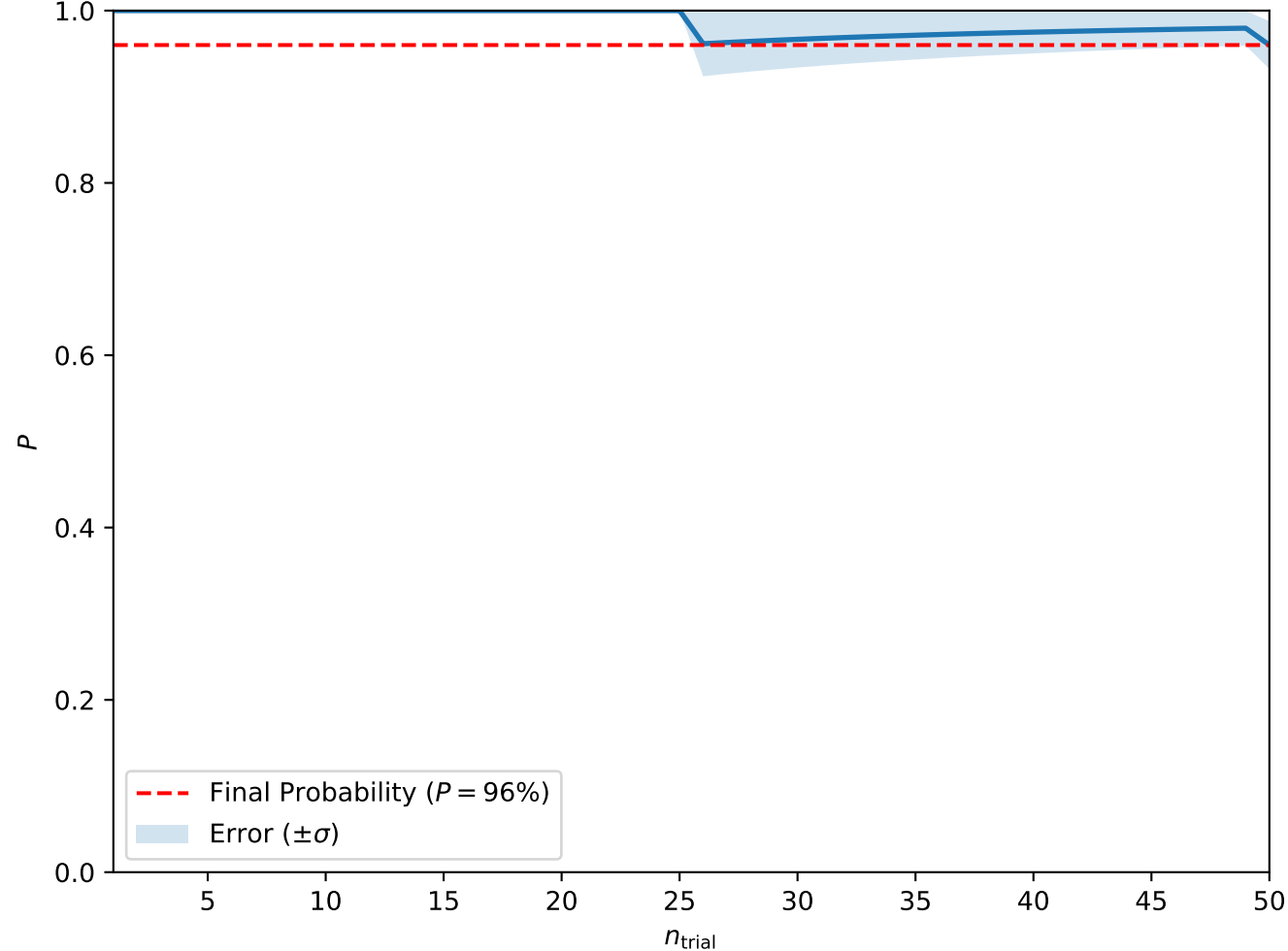
Convergence at A = 0.9, H = 0.3, T_0 = 1, w = 7.5 (Isolated Skyrmions)
