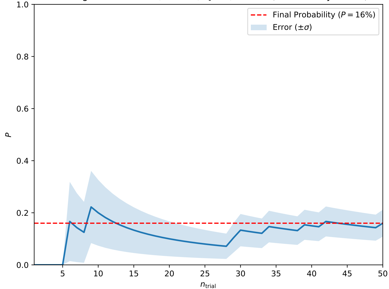
Convergence at A = 0.9, H = 0.3, T_0 = 3, w = 2.5 (Isolated Skyrmions)
