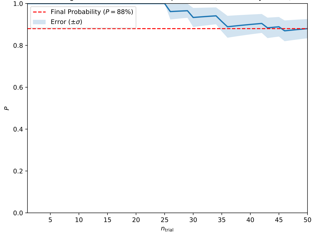
Convergence at A = 0.9, H = 0.3, T_0 = 3, w = 5 (Isolated Skyrmions)
