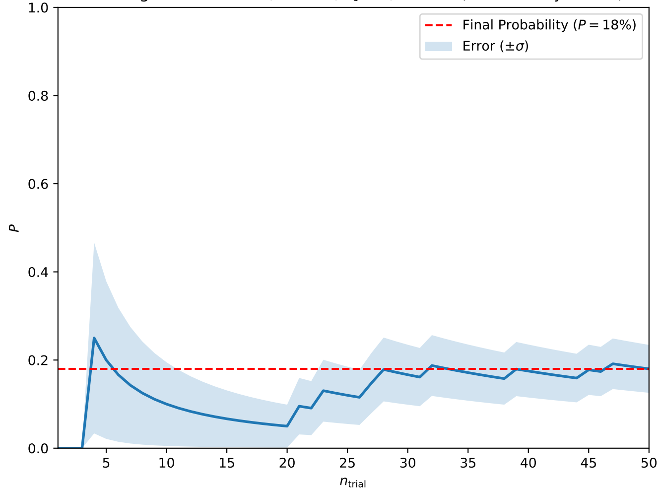
Convergence at A = 0.9, H = 0.3, T_0 = 5, w = 2.5 (Isolated Skyrmions)
