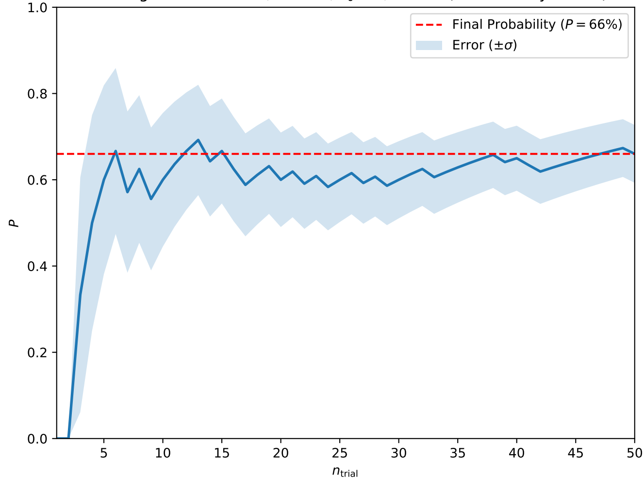
Convergence at A = 0.9, H = 0.4, T_0 = 1, w = 10 (Isolated Skyrmions)
