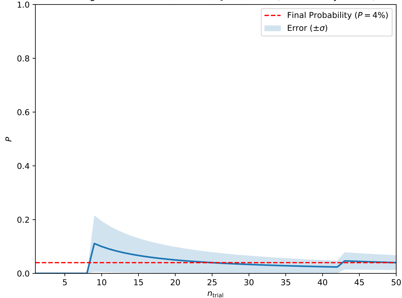
Convergence at A = 0.9, H = 0.4, T_0 = 1, w = 5 (Isolated Skyrmions)
