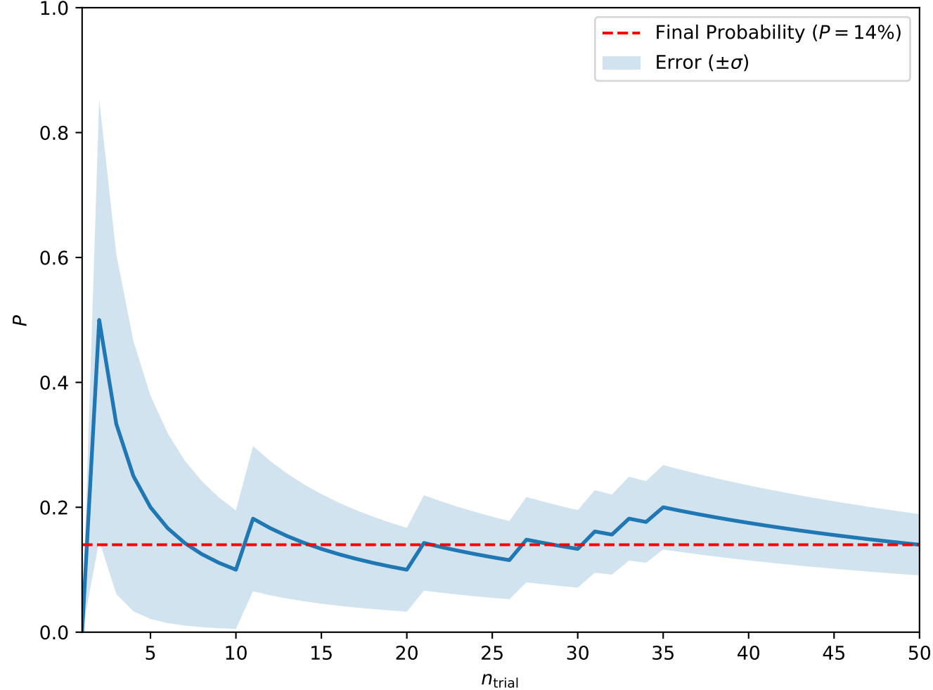
Convergence at A = 0.9, H = 0.4, T_0 = 1, w = 7.5 (Isolated Skyrmions)
