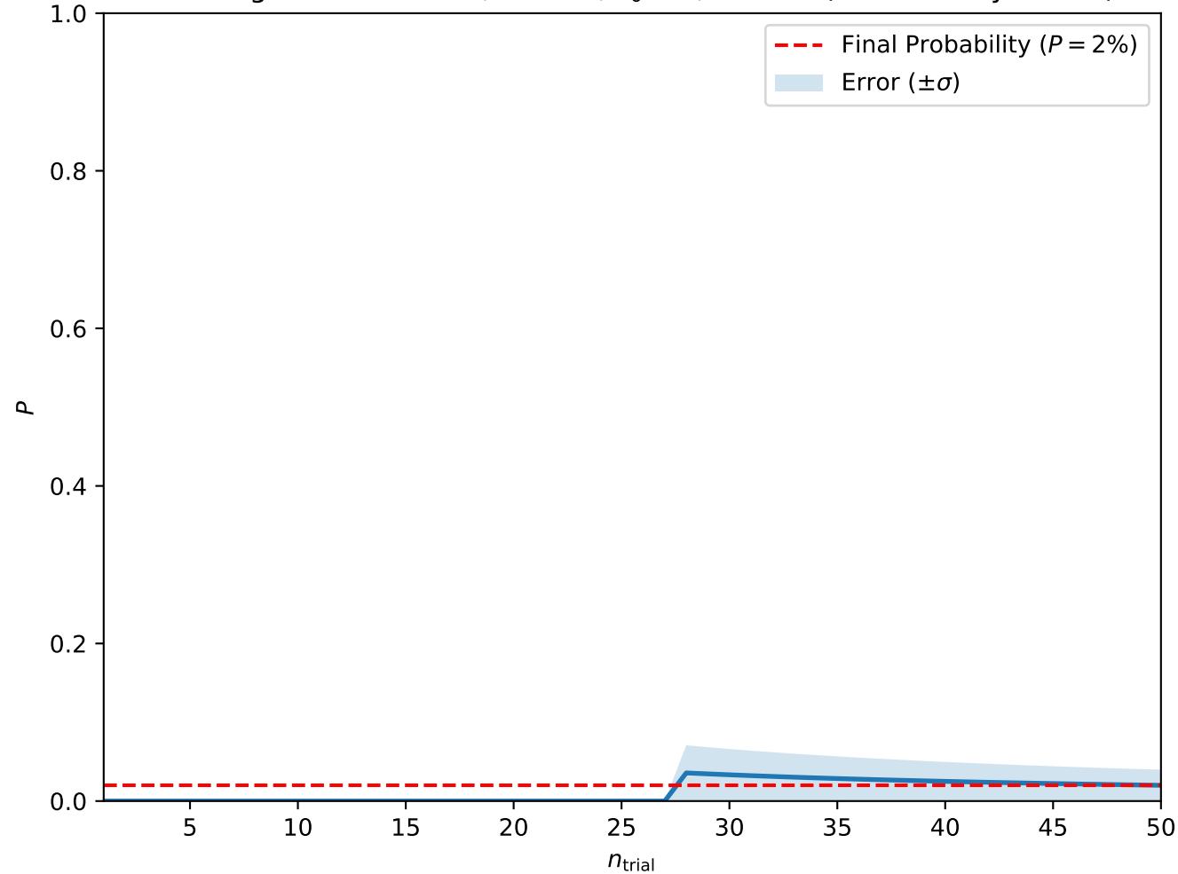
Convergence at A = 0.9, H = 0.4, T_0 = 3, w = 2.5 (Isolated Skyrmions)
