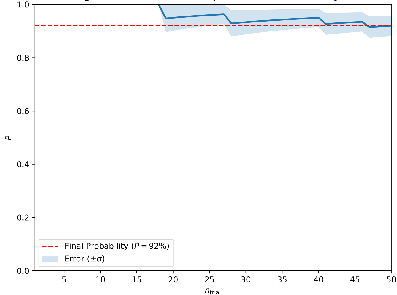
Convergence at A = 0.9, H = 0.4, T_0 = 3, w = 7.5 (Isolated Skyrmions)
