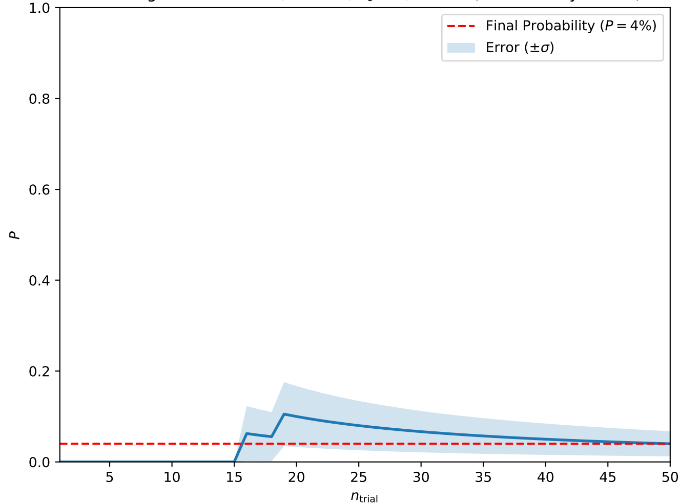
Convergence at A = 0.9, H = 0.5, T_0 = 1, w = 10 (Isolated Skyrmions)
