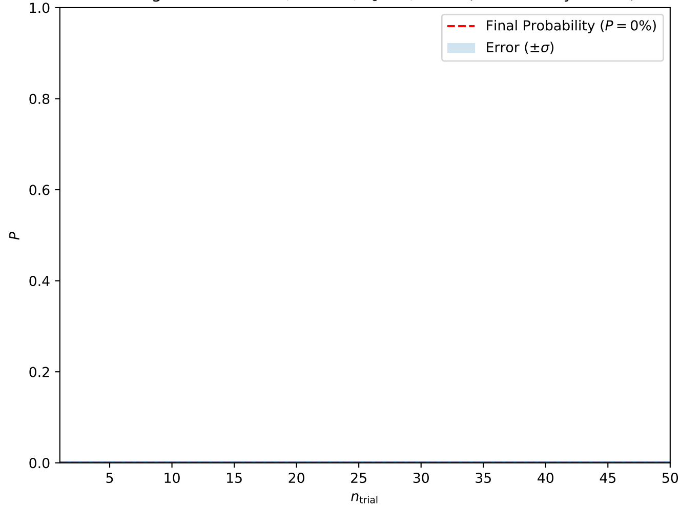
Convergence at A = 0.9, H = 0.5, T_0 = 1, w = 5 (Isolated Skyrmions)
