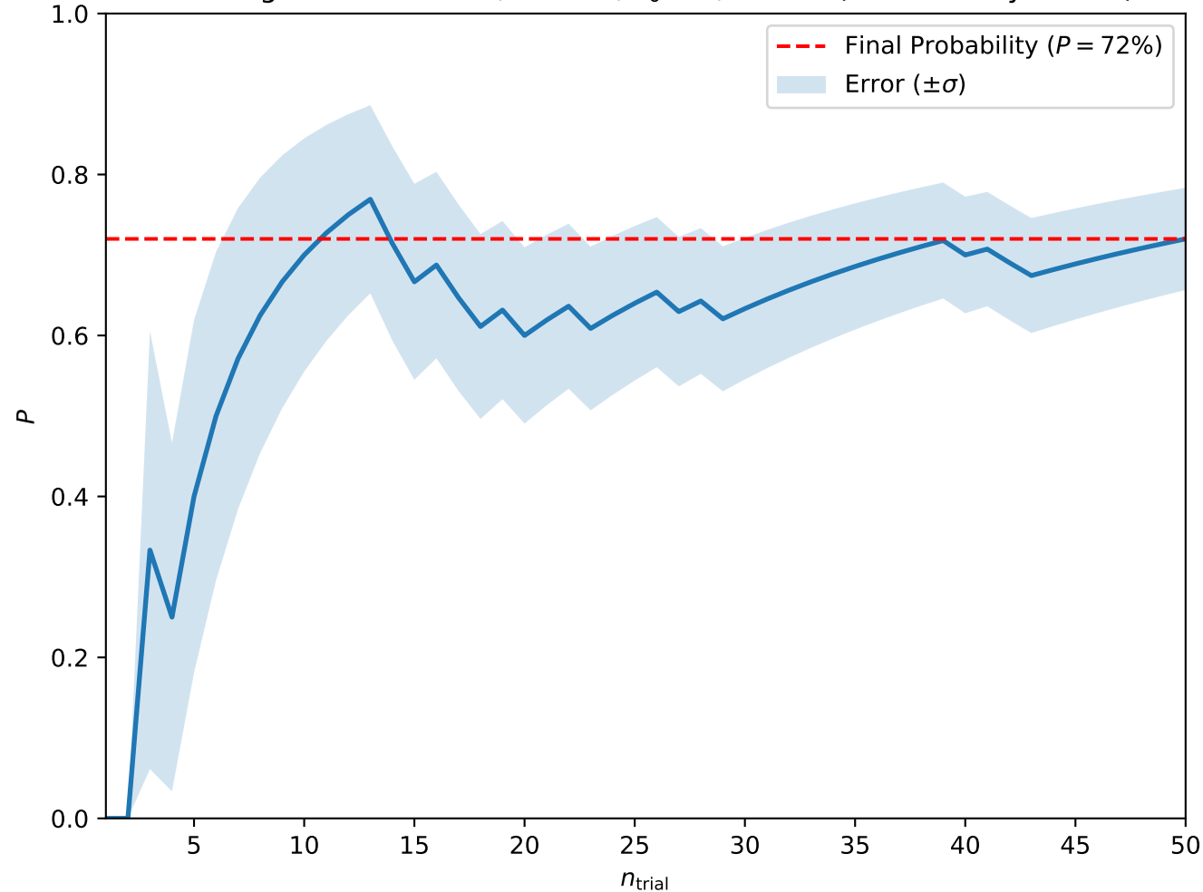
Convergence at A = 0.9, H = 0.5, T_0 = 3, w = 10 (Isolated Skyrmions)
