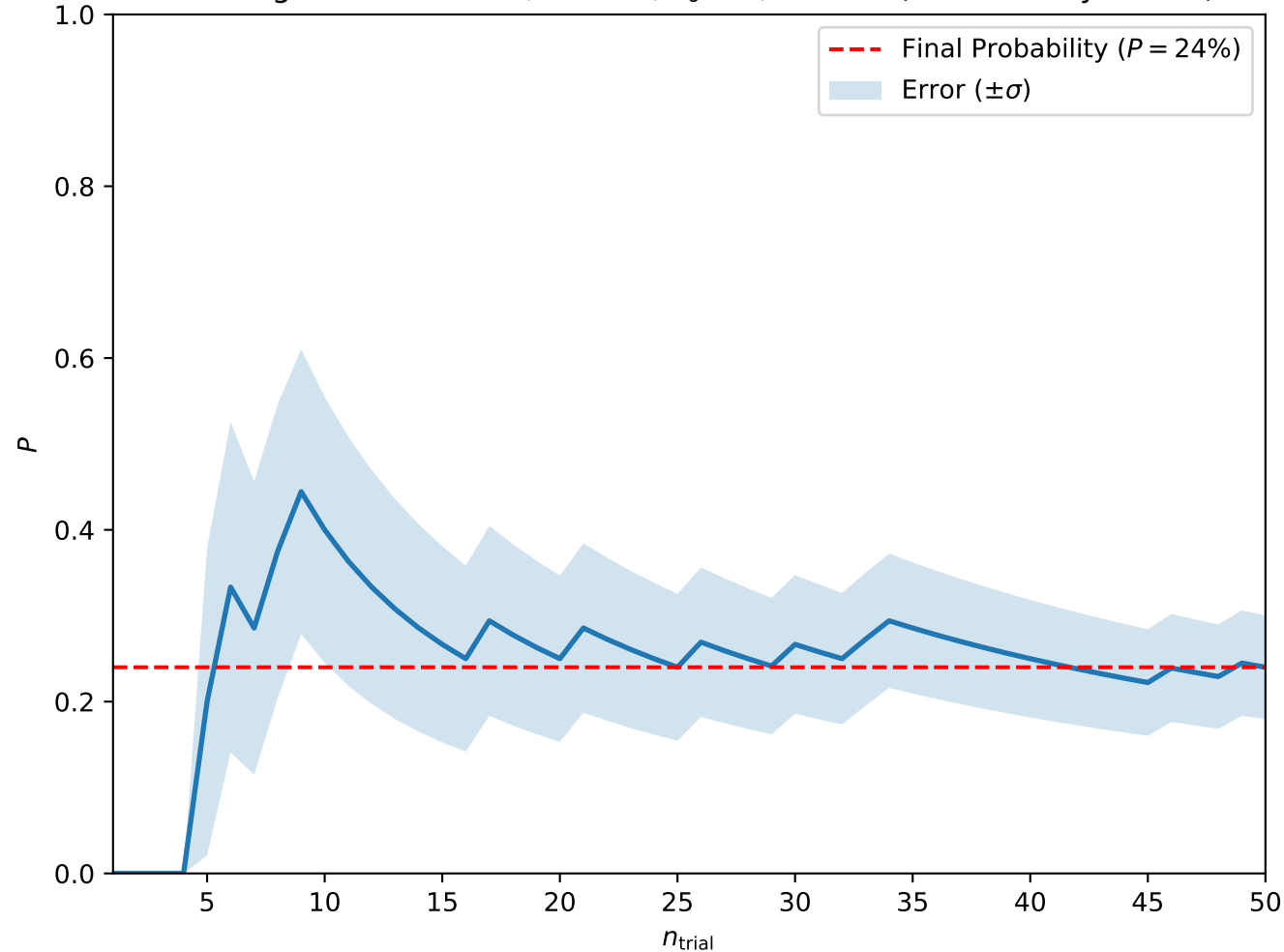
Convergence at A = 0.9, H = 0.5, T_0 = 3, w = 7.5 (Isolated Skyrmions)
