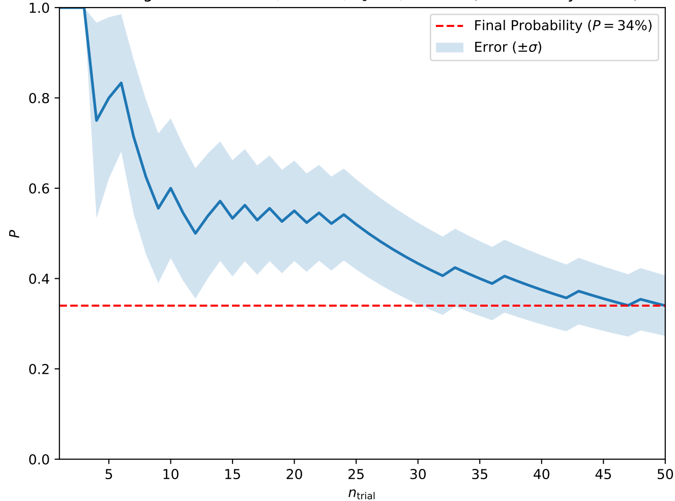
Convergence at A = 0.9, H = 0.5, T_0 = 5, w = 7.5 (Isolated Skyrmions)
