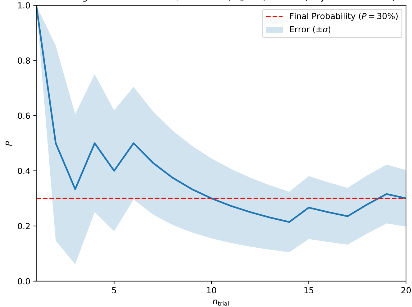
Convergence at A = 0.025, H = 0.225, T_0 = 3, w = 10 (Skyrmion Lattice)
