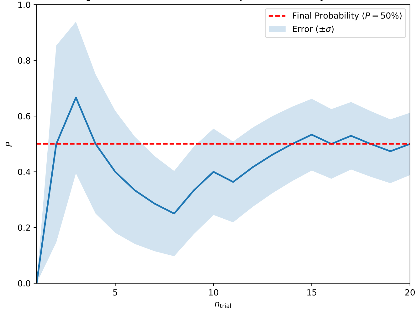
Convergence at A = 0.025, H = 0.25, T_0 = 3, w = 10 (Skyrmion Lattice)
