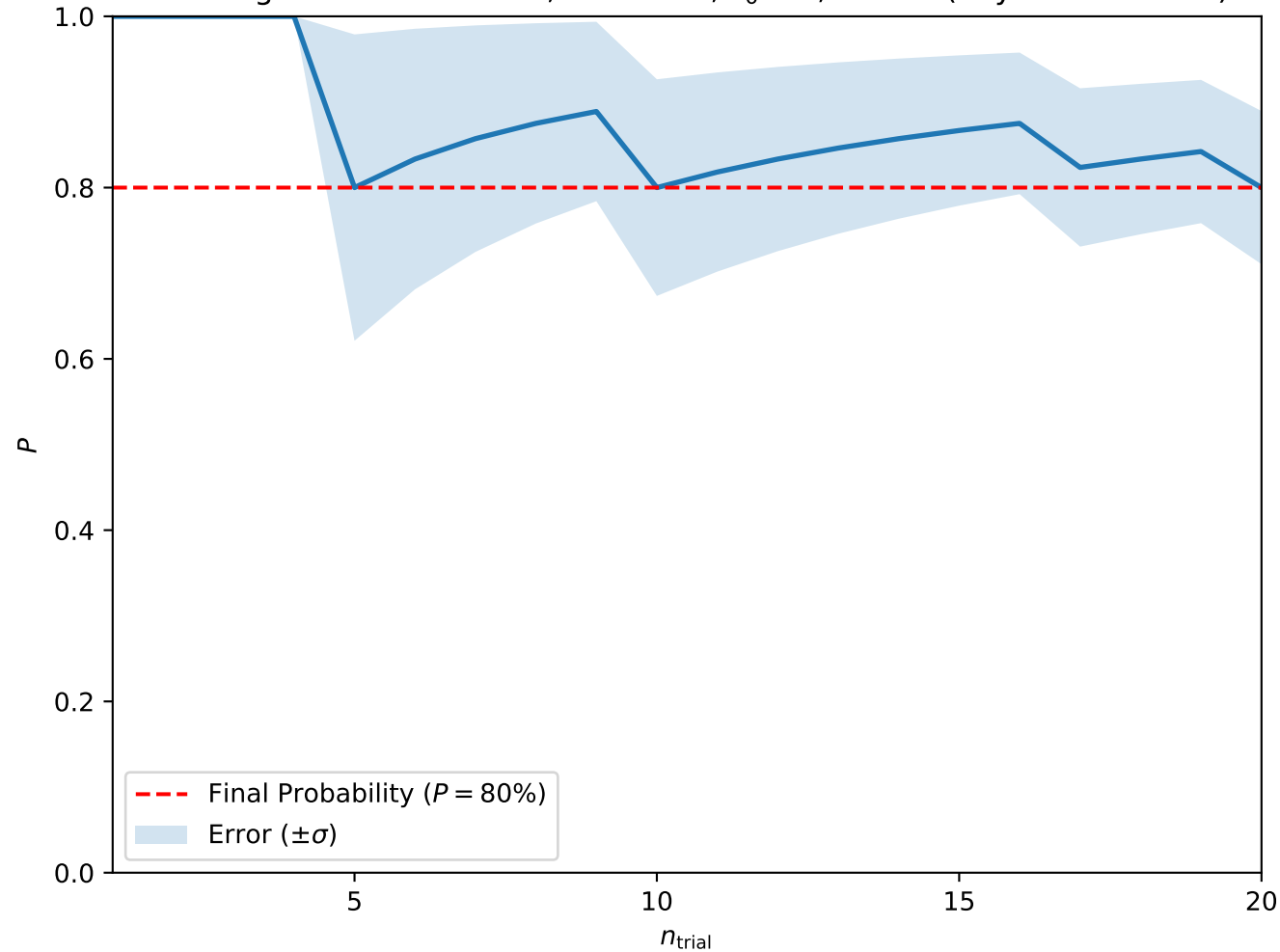
Convergence at A = 0.025, H = 0.275, T_0 = 3, w = 10 (Skyrmion Lattice)
