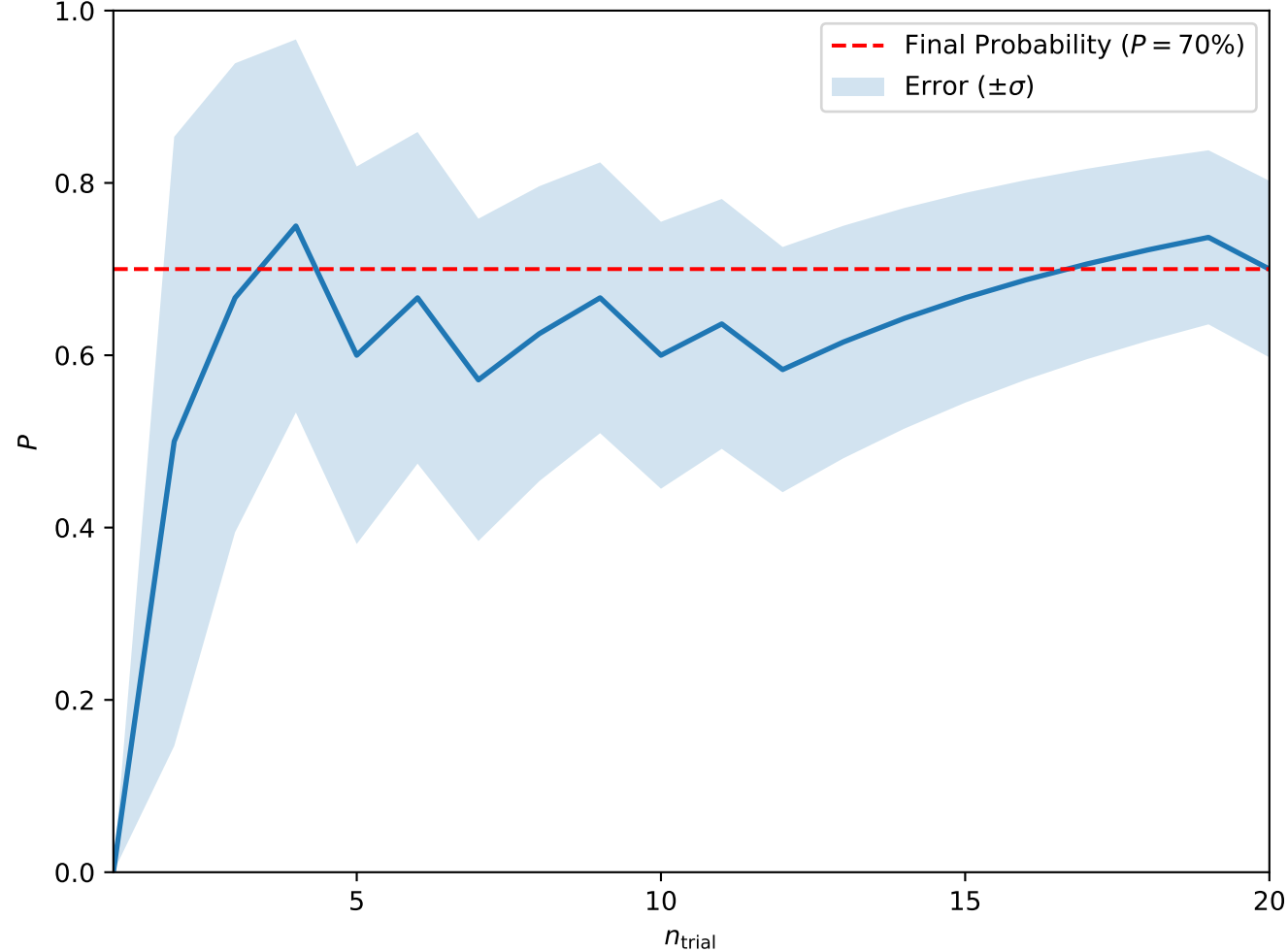
Convergence at A = 0.025, H = 0.3, T_0 = 3, w = 10 (Skyrmion Lattice)
