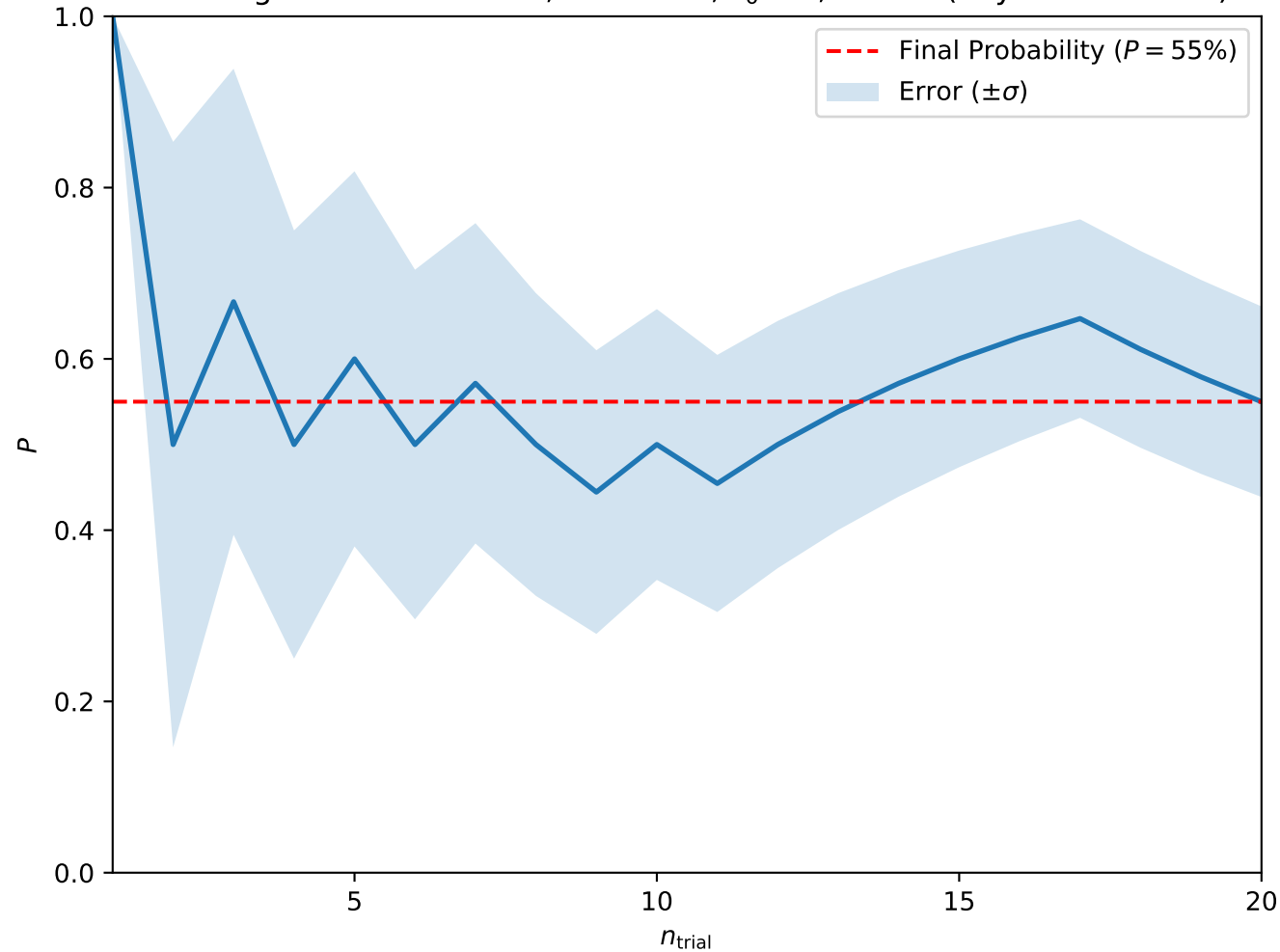
Convergence at A = 0.025, H = 0.325, T_0 = 3, w = 10 (Skyrmion Lattice)
