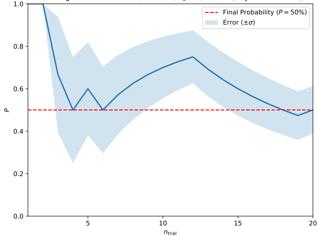
Convergence at A = 0.025, H = 0.35, T_0 = 3, w = 10 (Skyrmion Lattice)
