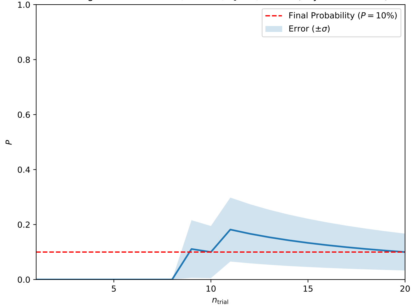
Convergence at A = 0.025, H = 0.4, T_0 = 3, w = 10 (Skyrmion Lattice)
