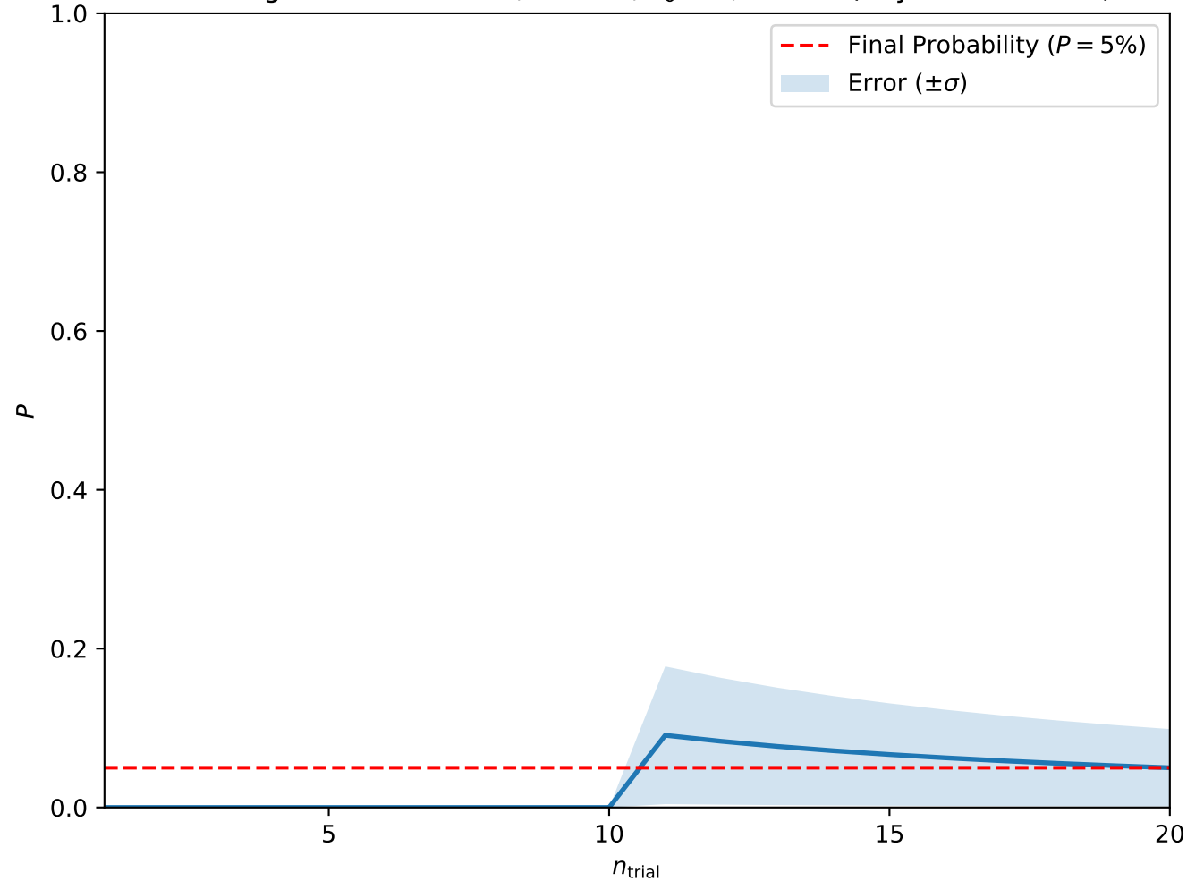
Convergence at A = 0.05, H = 0.2, T_0 = 3, w = 10 (Skyrmion Lattice)
