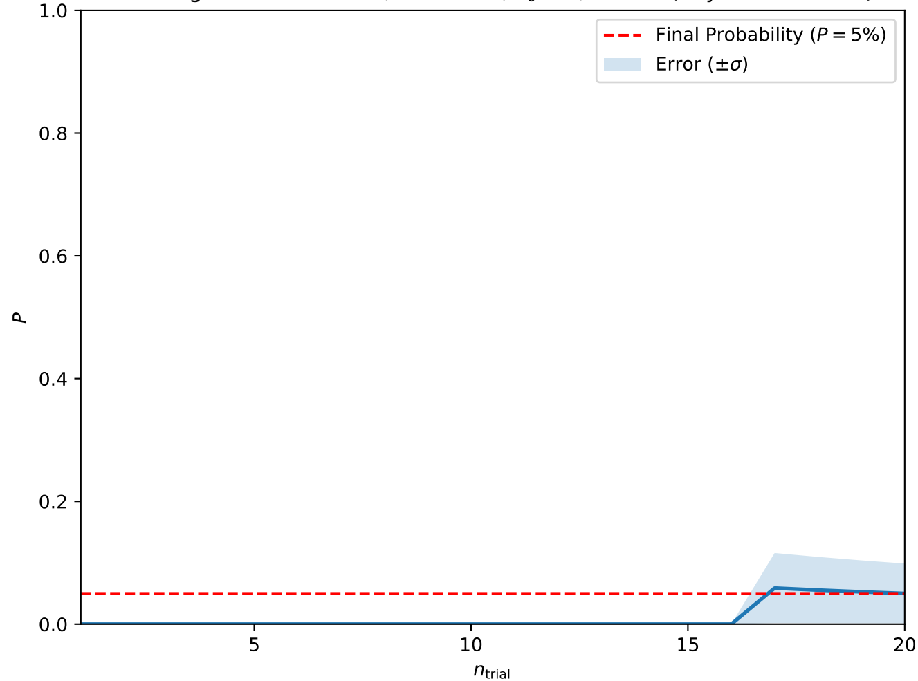
Convergence at A = 0.05, H = 0.225, T_0 = 3, w = 10 (Skyrmion Lattice)
