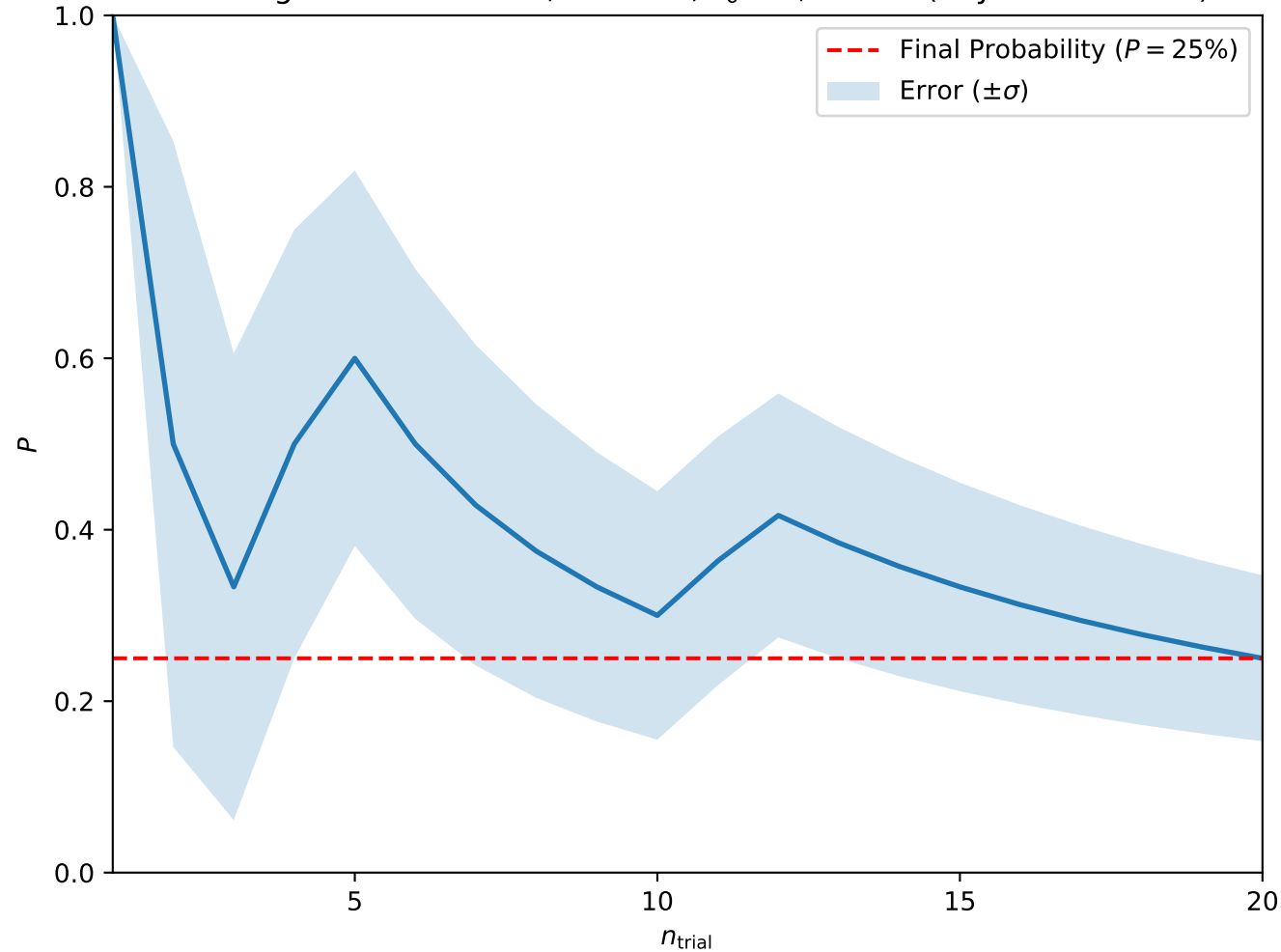
Convergence at A = 0.05, H = 0.25, T_0 = 3, w = 10 (Skyrmion Lattice)
