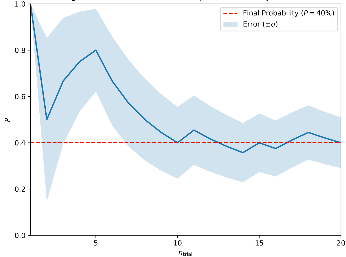
Convergence at A = 0.05, H = 0.275, T_0 = 3, w = 10 (Skyrmion Lattice)
